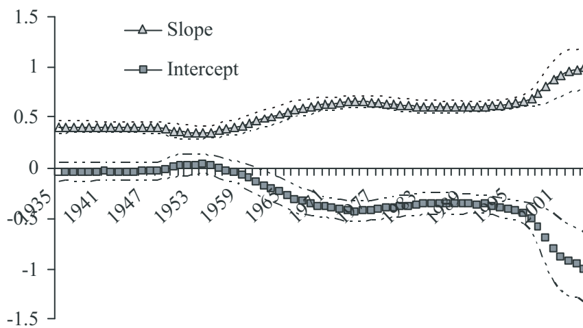
Figure 3. Incremental Regression Coefficients and 2SE Bands 1935-2004 (rescaled).
