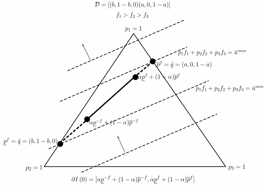
Figure 3: \mathcal{D} has less than full rank
