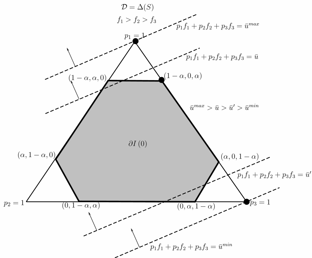
Figure 2: \mathcal{D} has full rank
