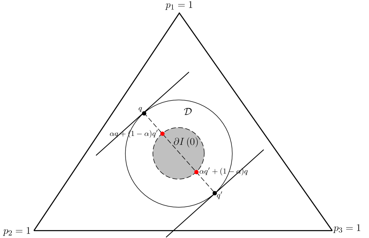
Figure 1: Circular set of priors
