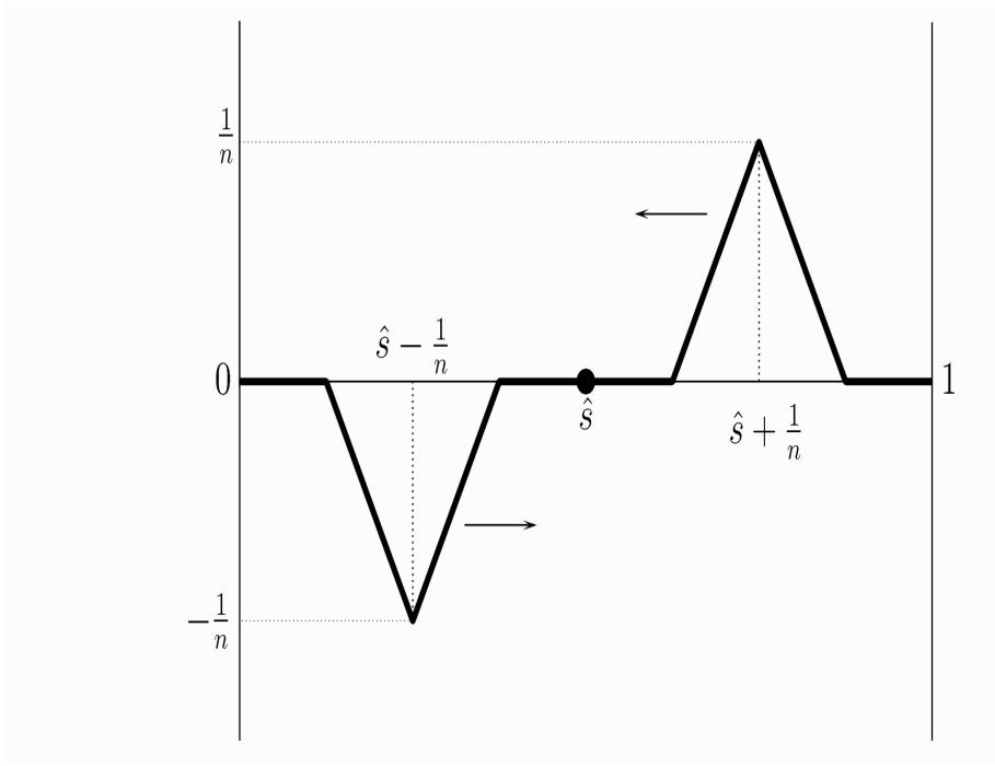
Figure 4: The function f_n
